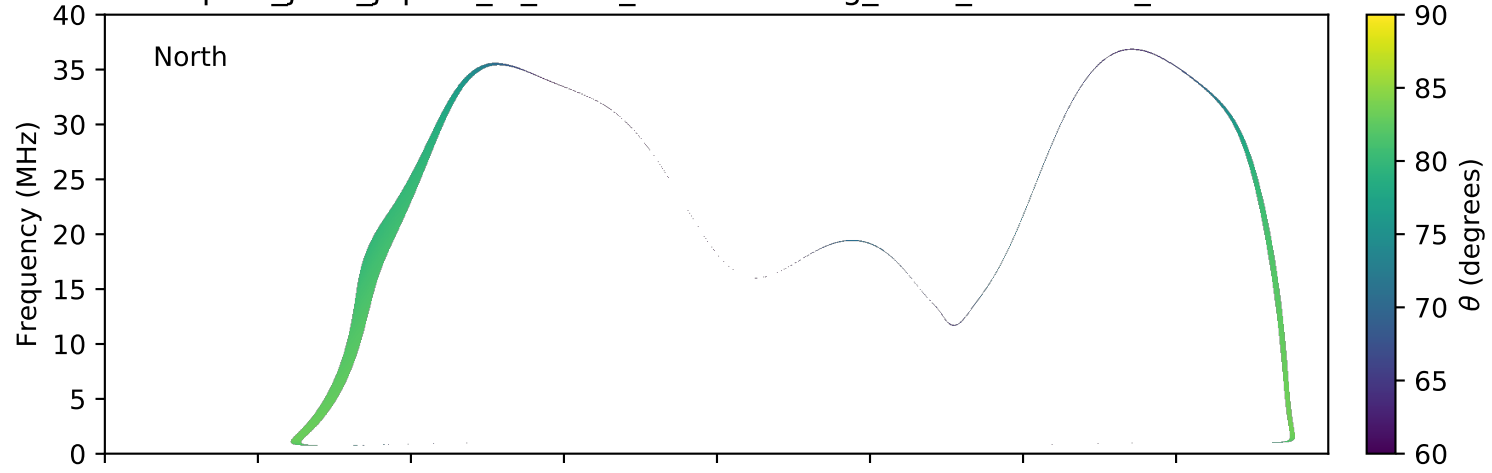
expres_juno_jupiter_io_isaac_lossc-wid1deg_3kev_20160808_v01.cdf
