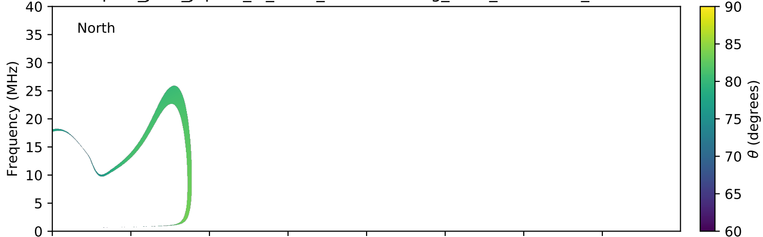
expres_juno_jupiter_io_isaac_lossc-wid1deg_3kev_20160807_v01.cdf
