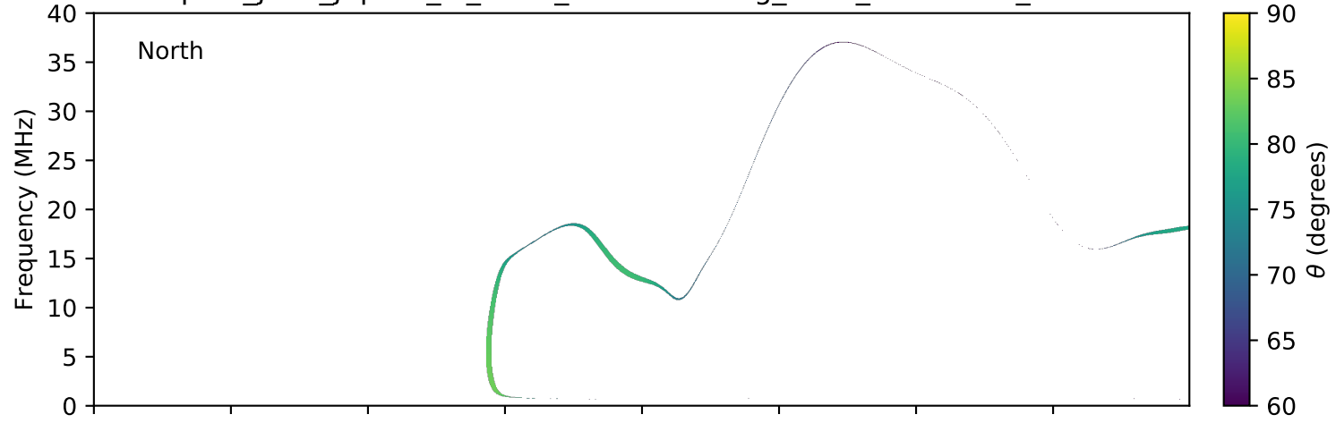
expres_juno_jupiter_io_isaac_lossc-wid1deg_3kev_20160806_v01.cdf
