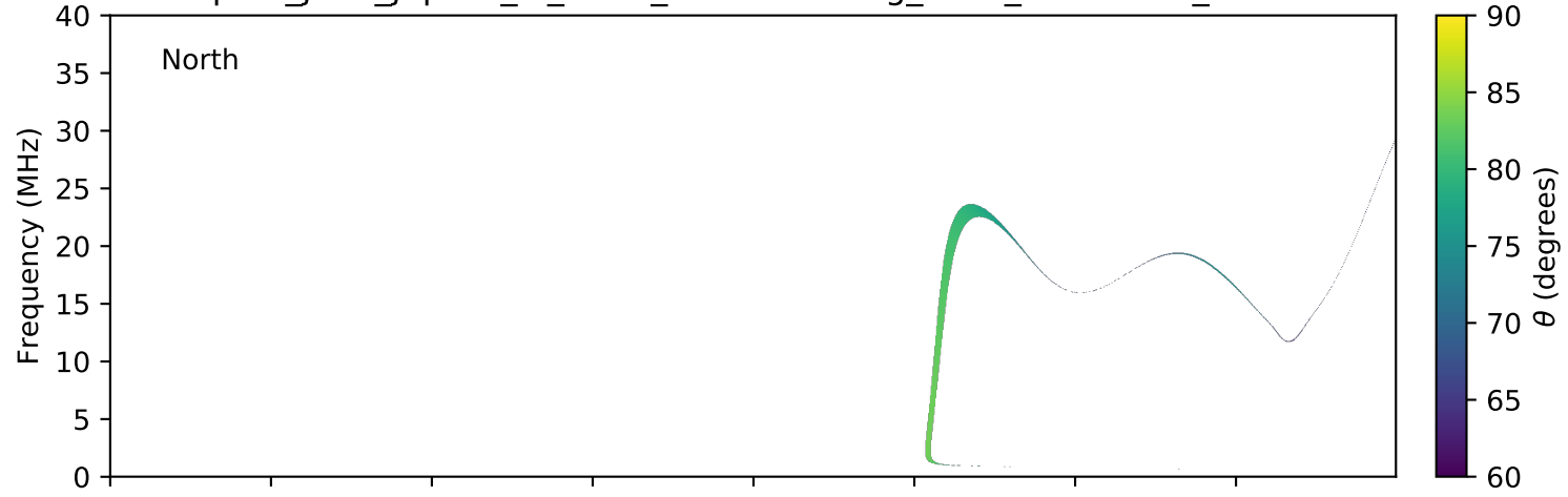
expres_juno_jupiter_io_isaac_lossc-wid1deg_3kev_20160804_v01.cdf
