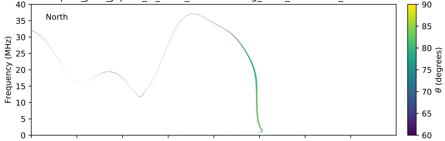
expres_juno_jupiter_io_isaac_lossc-wid1deg_3kev_20160803_v01.cdf
