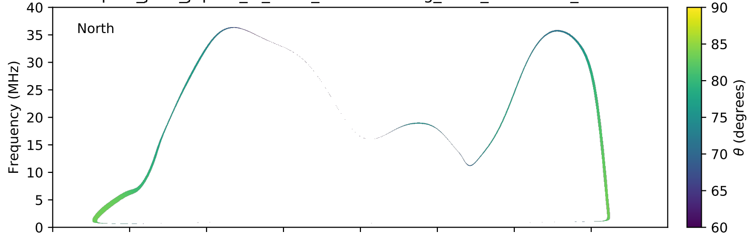
expres_juno_jupiter_io_isaac_lossc-wid1deg_3kev_20160801_v01.cdf
