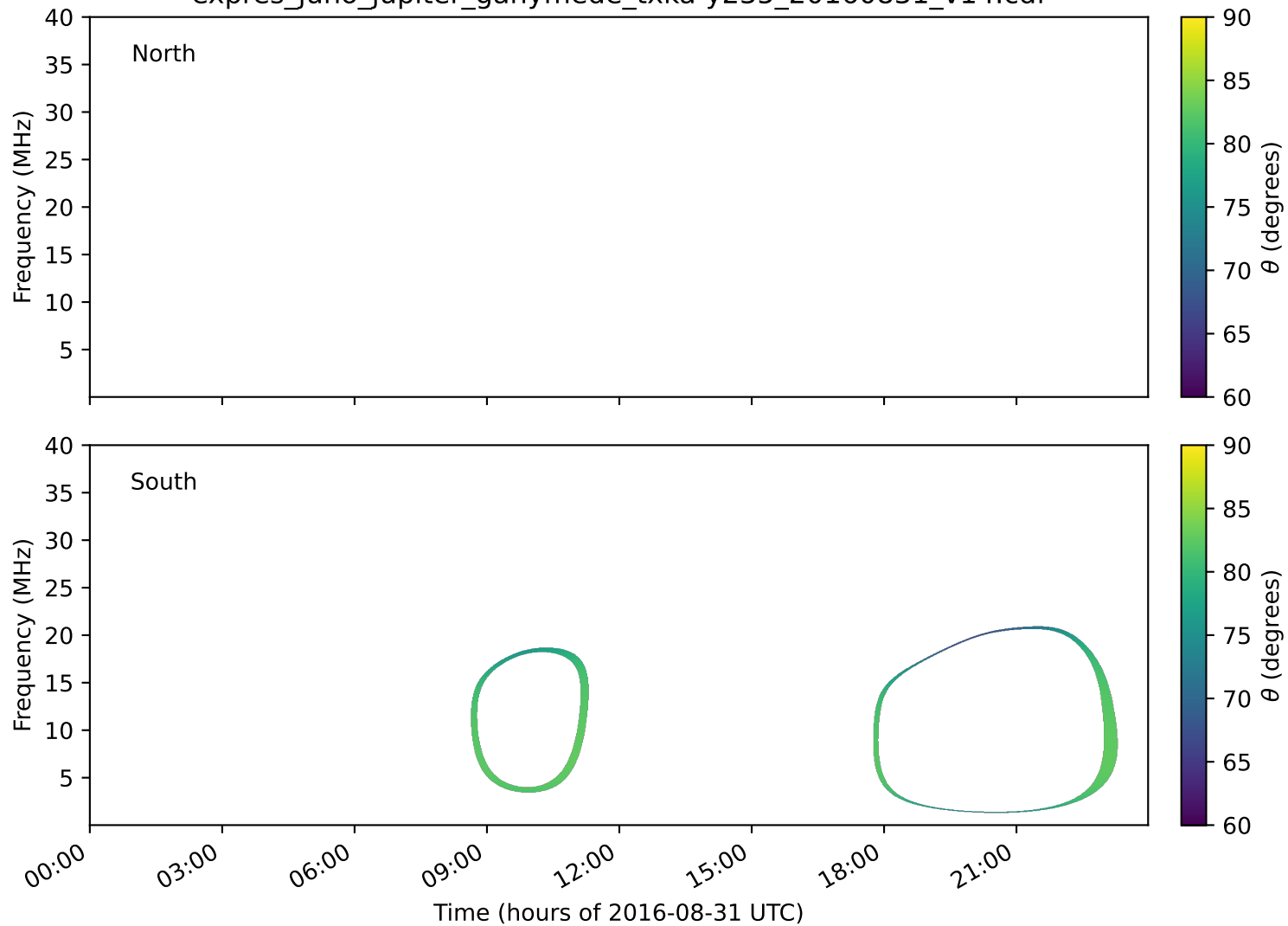
expres_juno_jupiter_ganymede_txka-y235_20160831_v14.cdf
