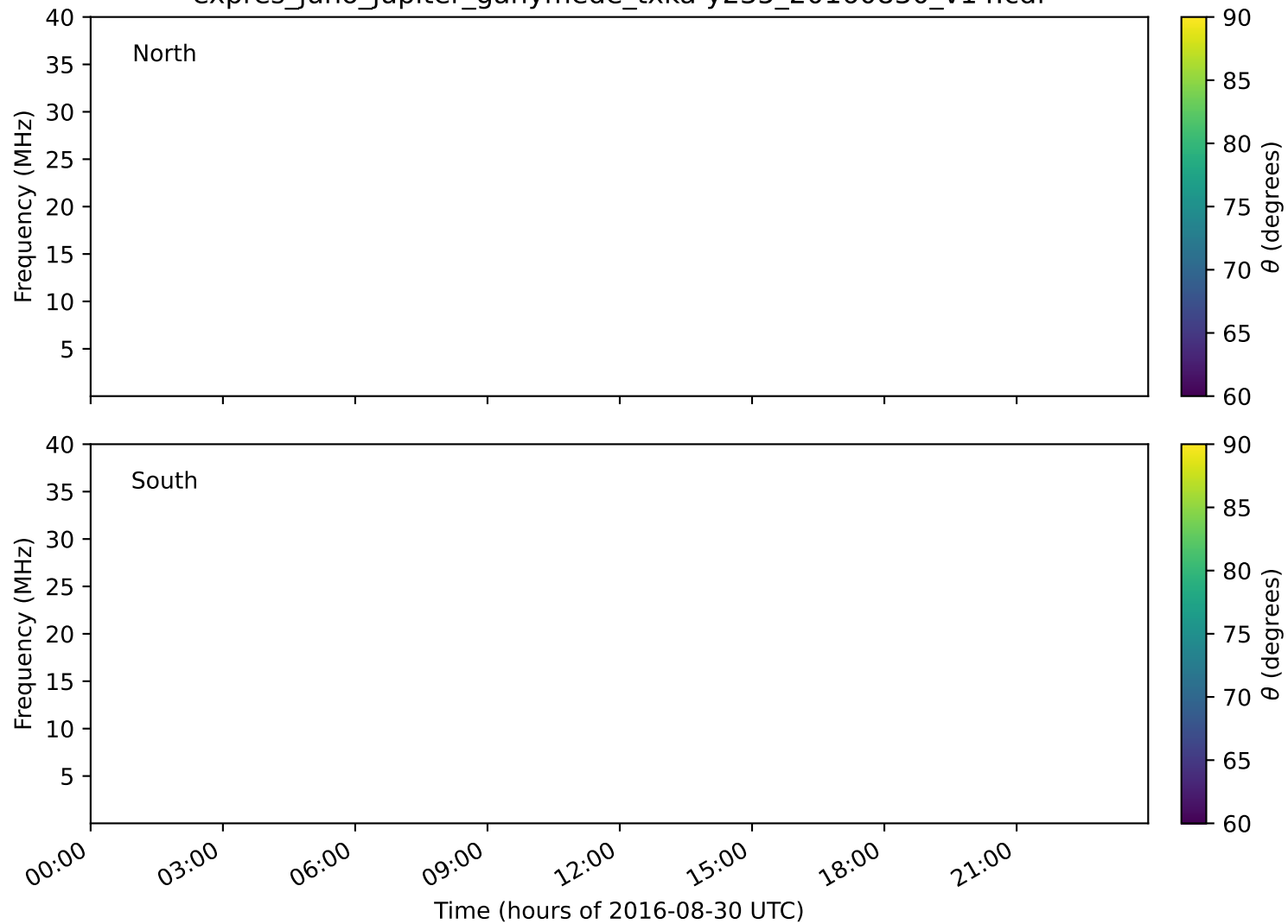
expres_juno_jupiter_ganymede_txka-y235_20160830_v14.cdf
