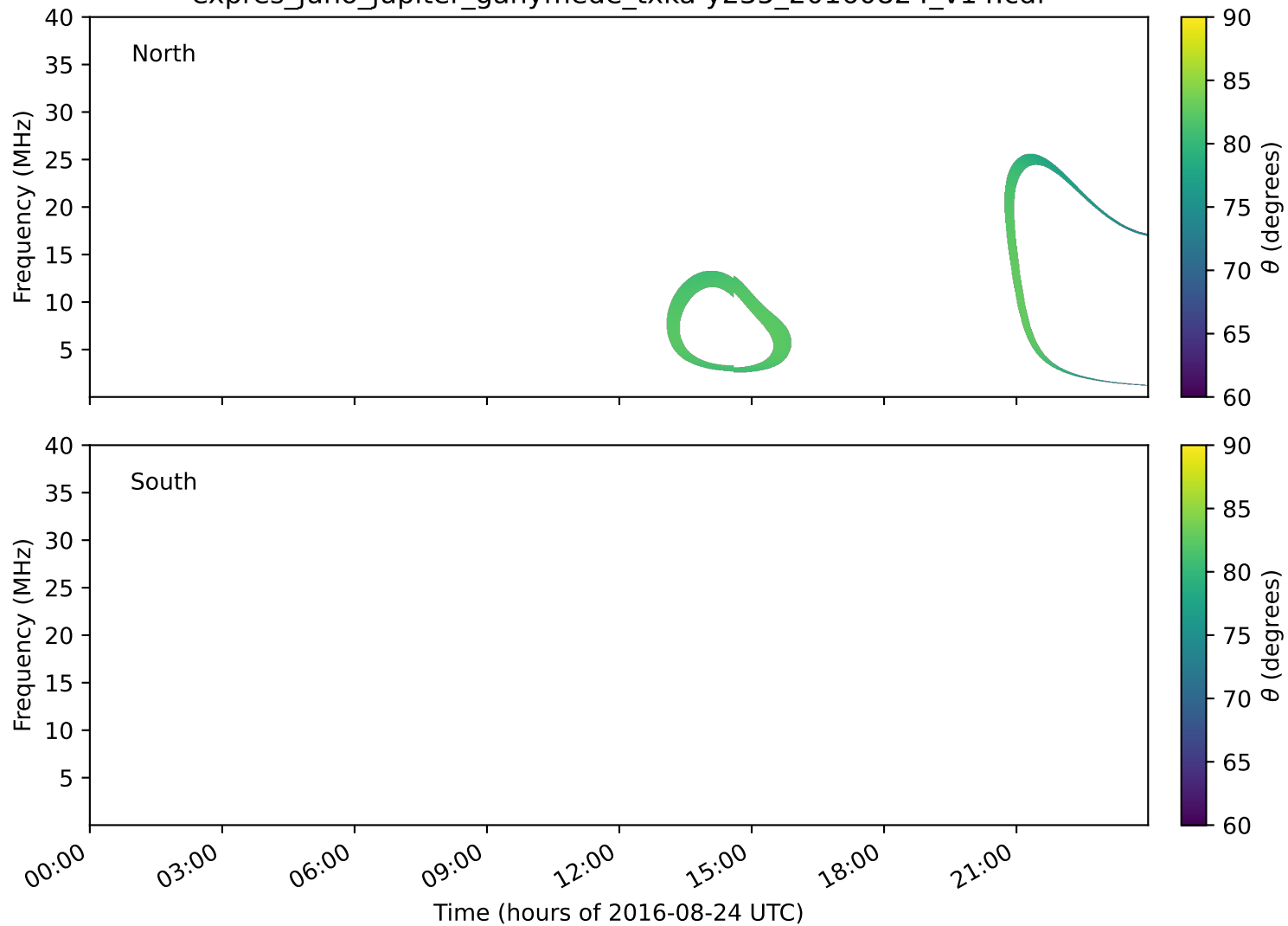
expres_juno_jupiter_ganymede_txka-y235_20160824_v14.cdf
