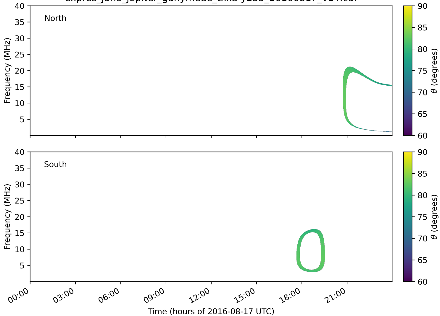
expres_juno_jupiter_ganymede_txka-y235_20160817_v14.cdf
