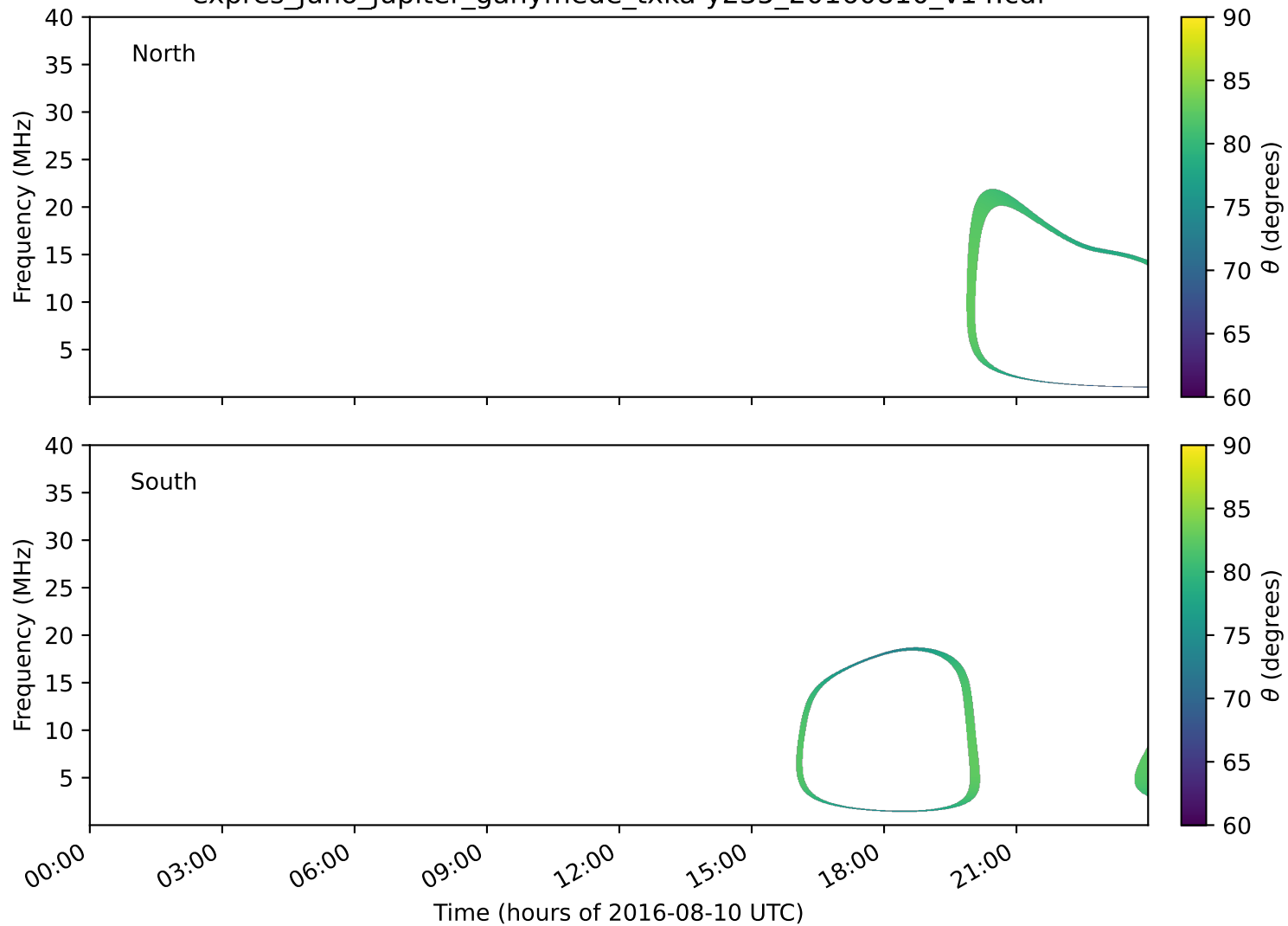
expres_juno_jupiter_ganymede_txka-y235_20160810_v14.cdf
