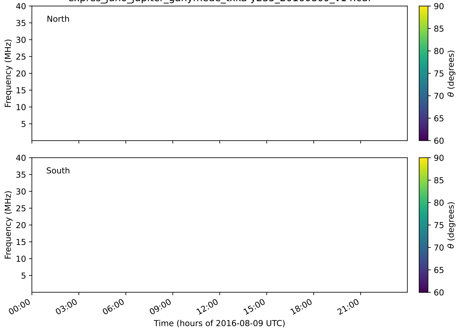
expres_juno_jupiter_ganymede_txka-y235_20160809_v14.cdf
