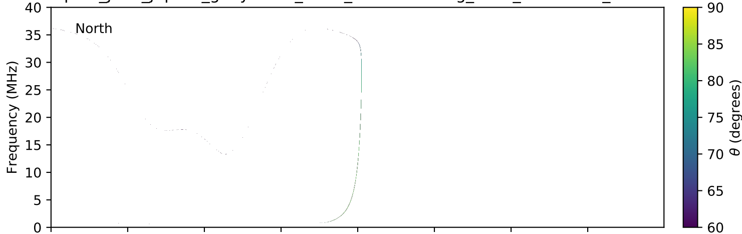
expres_juno_jupiter_ganymede_isaac_lossc-wid1deg_3kev_20160827_v01.cdf
