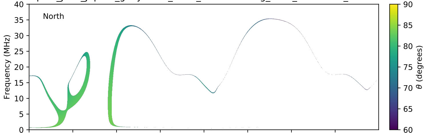
expres_juno_jupiter_ganymede_isaac_lossc-wid1deg_3kev_20160825_v01.cdf
