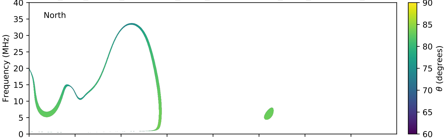
expres_juno_jupiter_ganymede_isaac_lossc-wid1deg_3kev_20160821_v01.cdf
