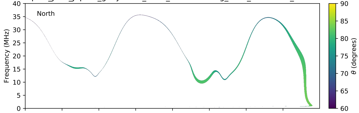
expres_juno_jupiter_ganymede_isaac_lossc-wid1deg_3kev_20160813_v01.cdf
