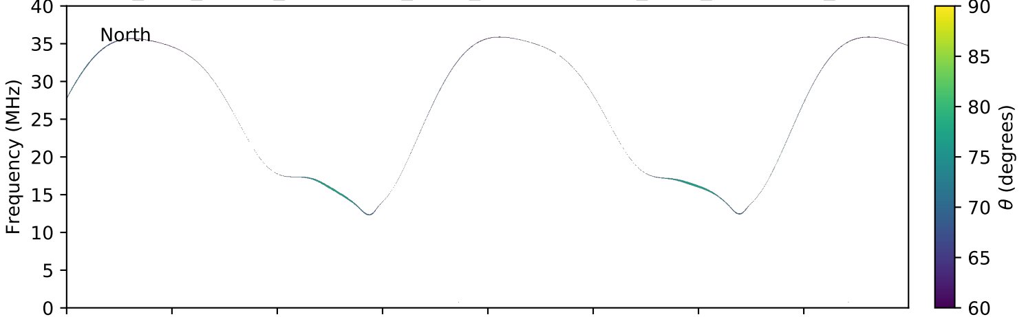
expres_juno_jupiter_ganymede_isaac_lossc-wid1deg_3kev_20160812_v01.cdf
