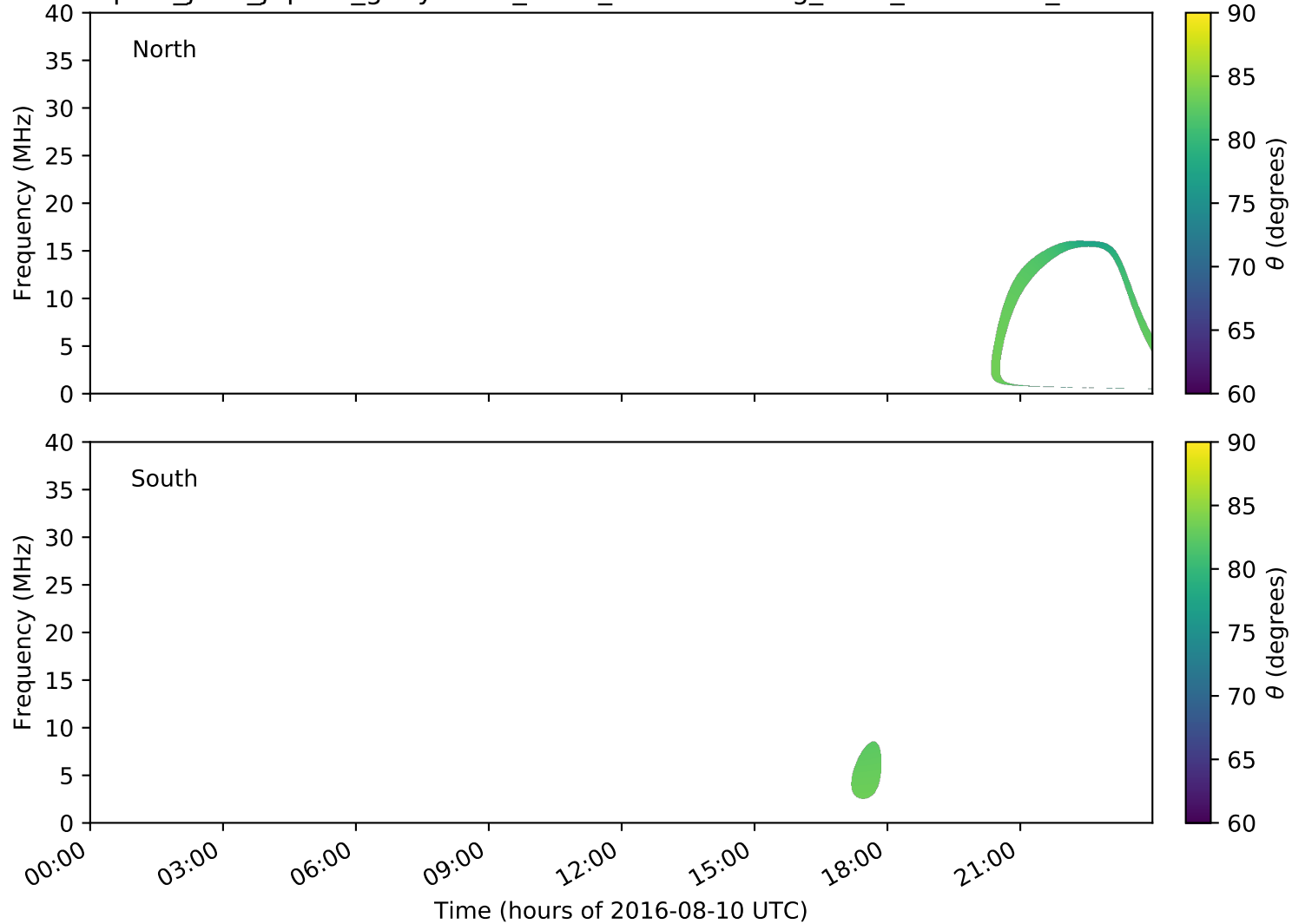
expres_juno_jupiter_ganymede_isaac_lossc-wid1deg_3kev_20160810_v01.cdf
