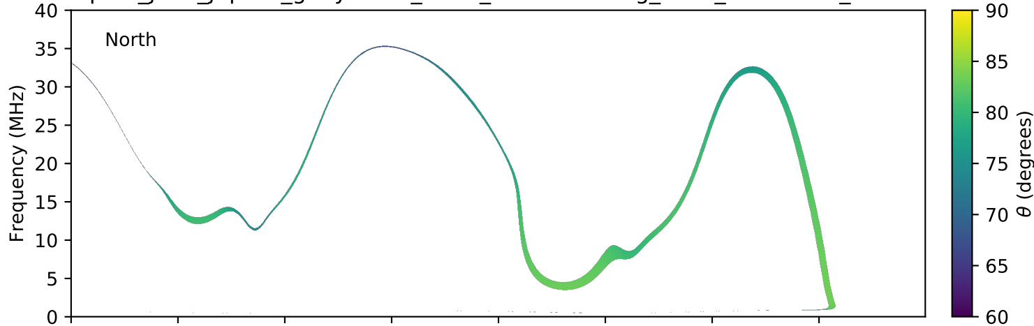
expres_juno_jupiter_ganymede_isaac_lossc-wid1deg_3kev_20160806_v01.cdf
