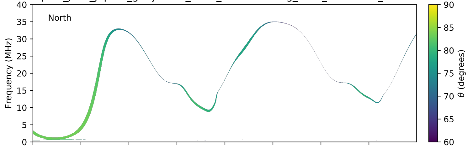
expres_juno_jupiter_ganymede_isaac_lossc-wid1deg_3kev_20160804_v01.cdf
