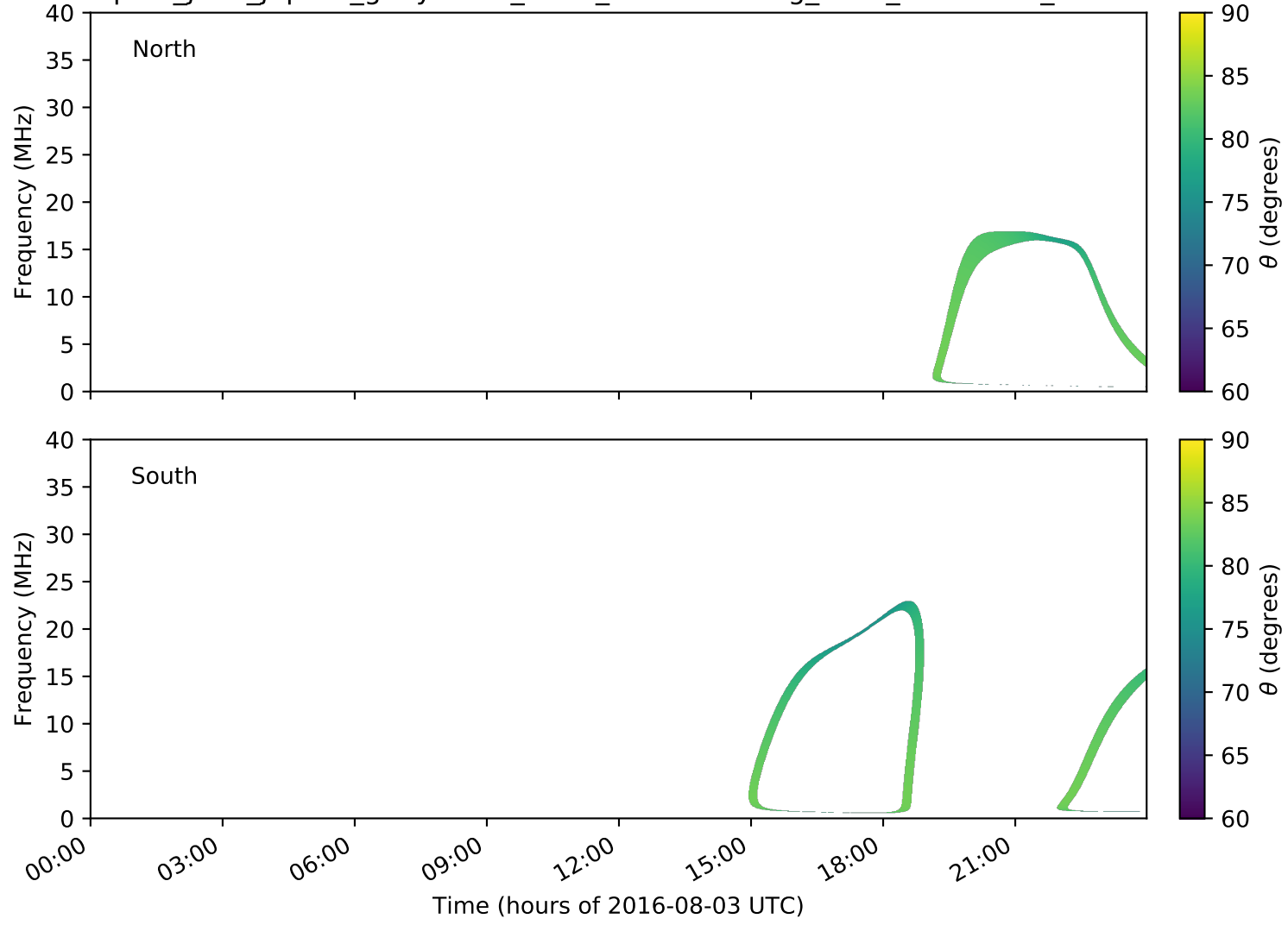
expres_juno_jupiter_ganymede_isaac_lossc-wid1deg_3kev_20160803_v01.cdf
