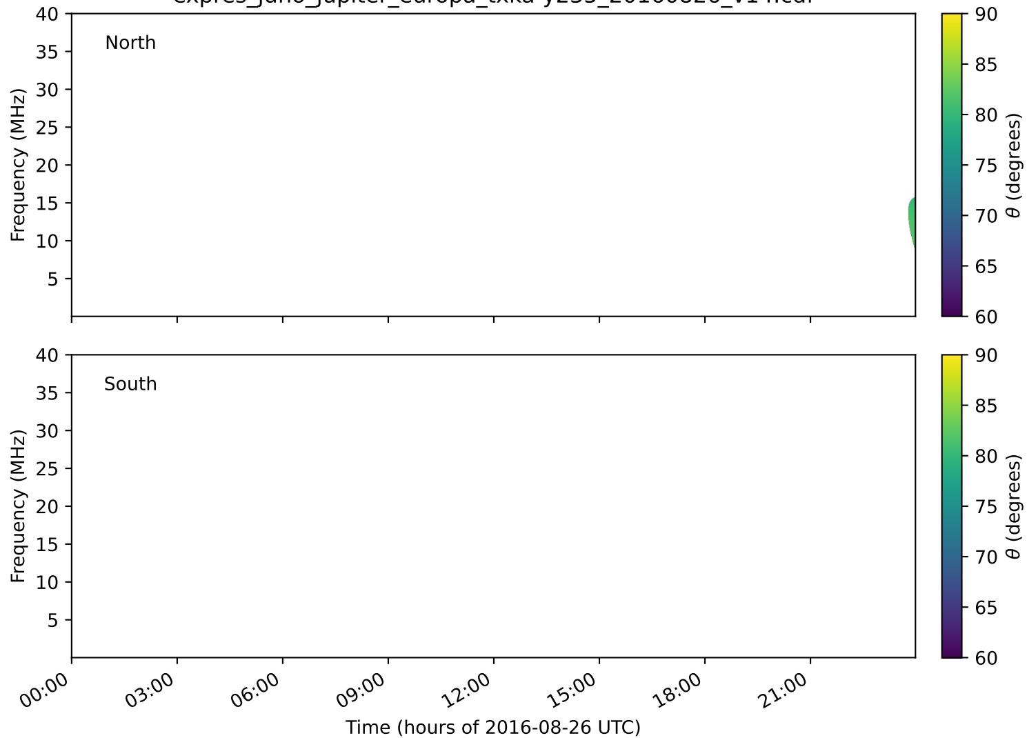
expres_juno_jupiter_europa_txka-y235_20160826_v14.cdf
