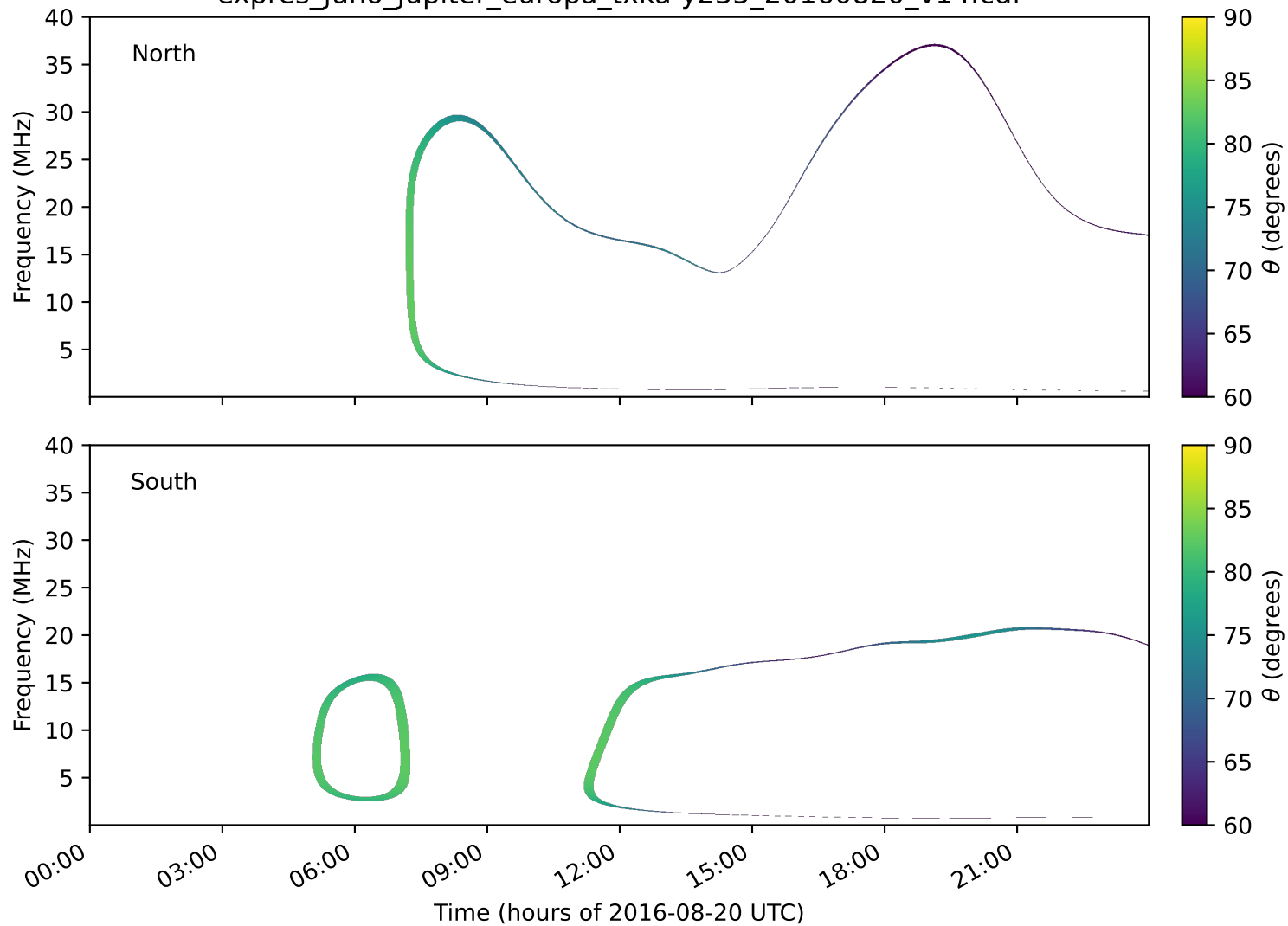
expres_juno_jupiter_europa_txka-y235_20160820_v14.cdf
