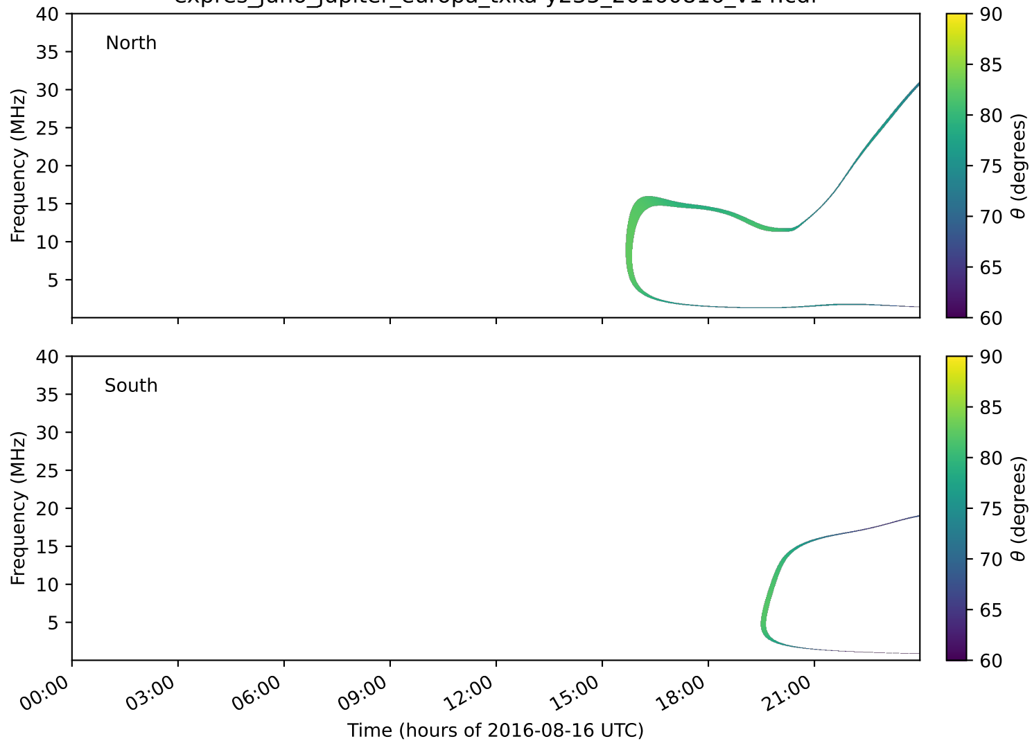
expres_juno_jupiter_europa_txka-y235_20160816_v14.cdf
