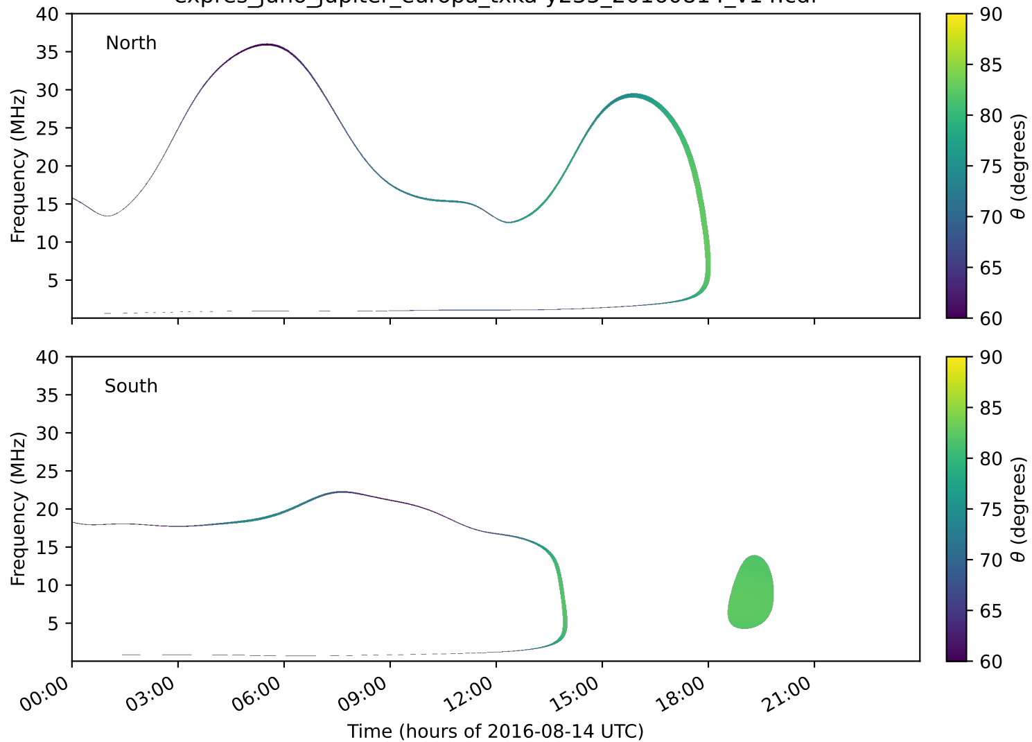
expres_juno_jupiter_europa_txka-y235_20160814_v14.cdf
