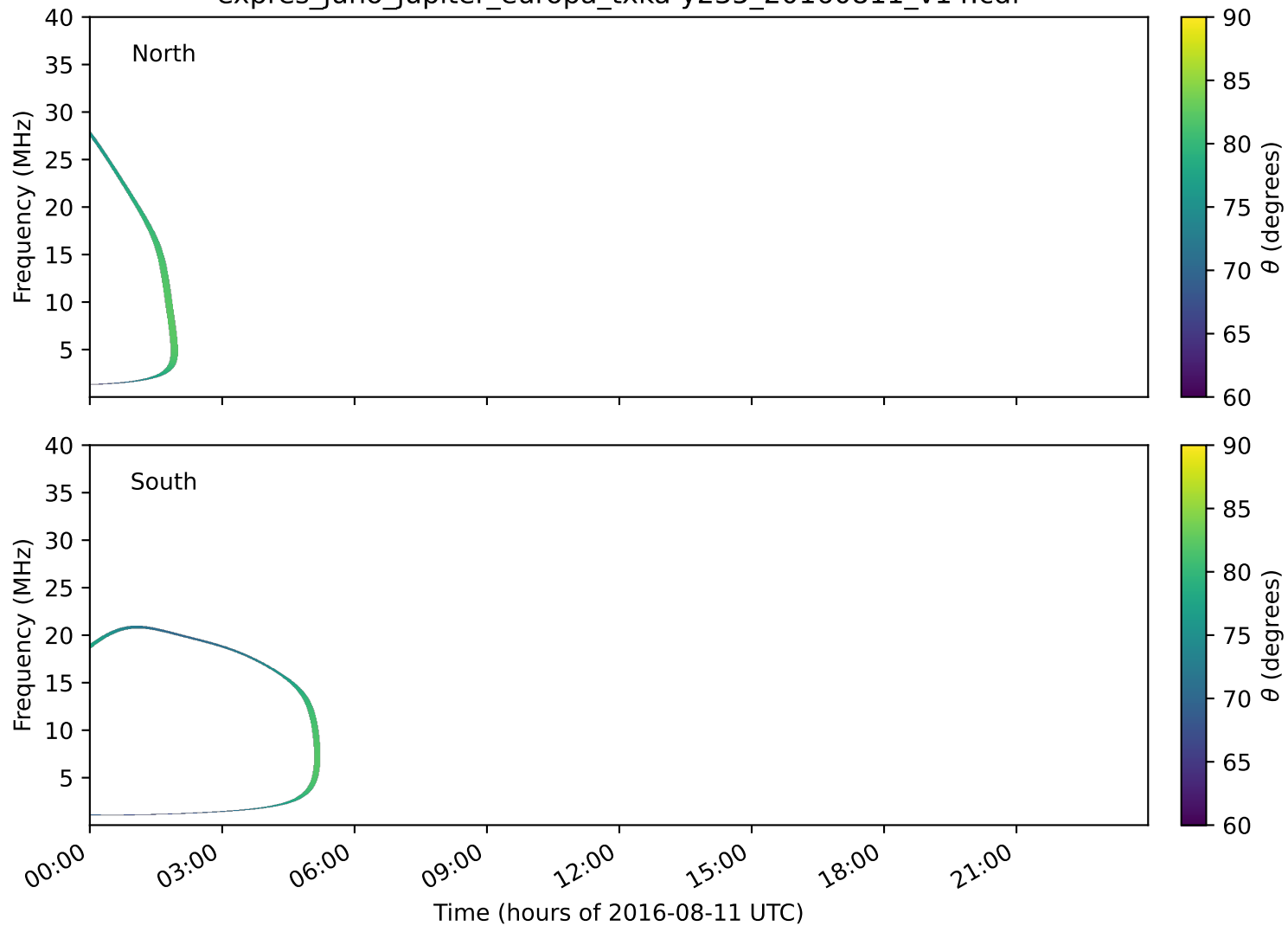
expres_juno_jupiter_europa_txka-y235_20160811_v14.cdf
