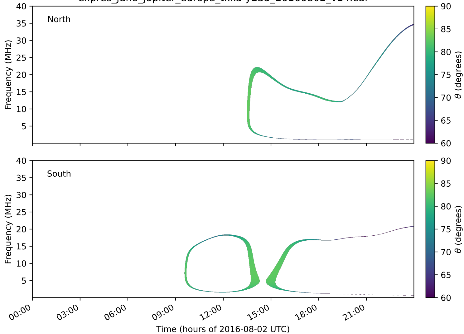
expres_juno_jupiter_europa_txka-y235_20160802_v14.cdf
