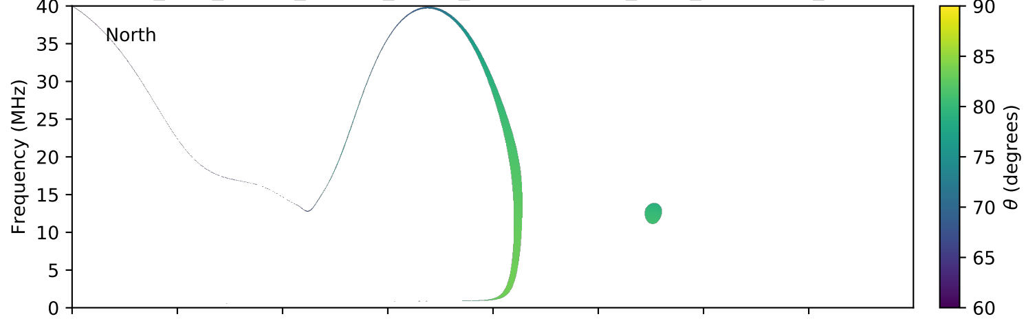
expres_juno_jupiter_europa_jrm09_lossc-wid1deg_3kev_20160825_v01.cdf
