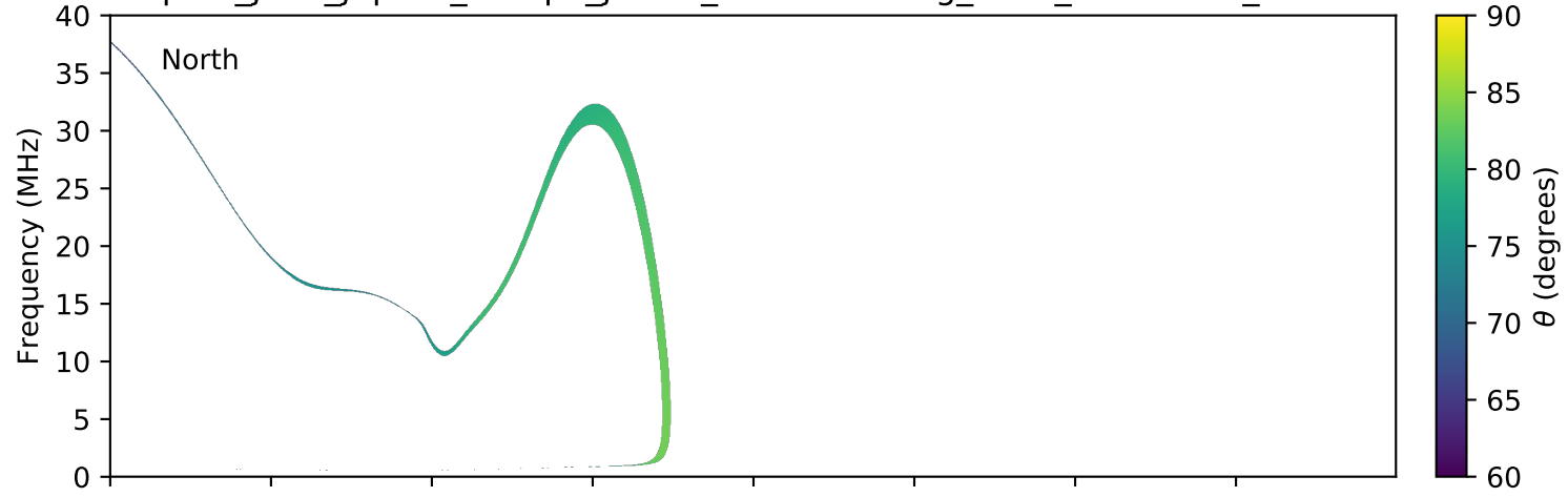
expres_juno_jupiter_europa_jrm09_lossc-wid1deg_3kev_20160818_v01.cdf
