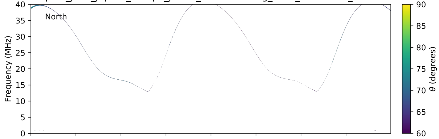
expres_juno_jupiter_europa_jrm09_lossc-wid1deg_3kev_20160817_v01.cdf
