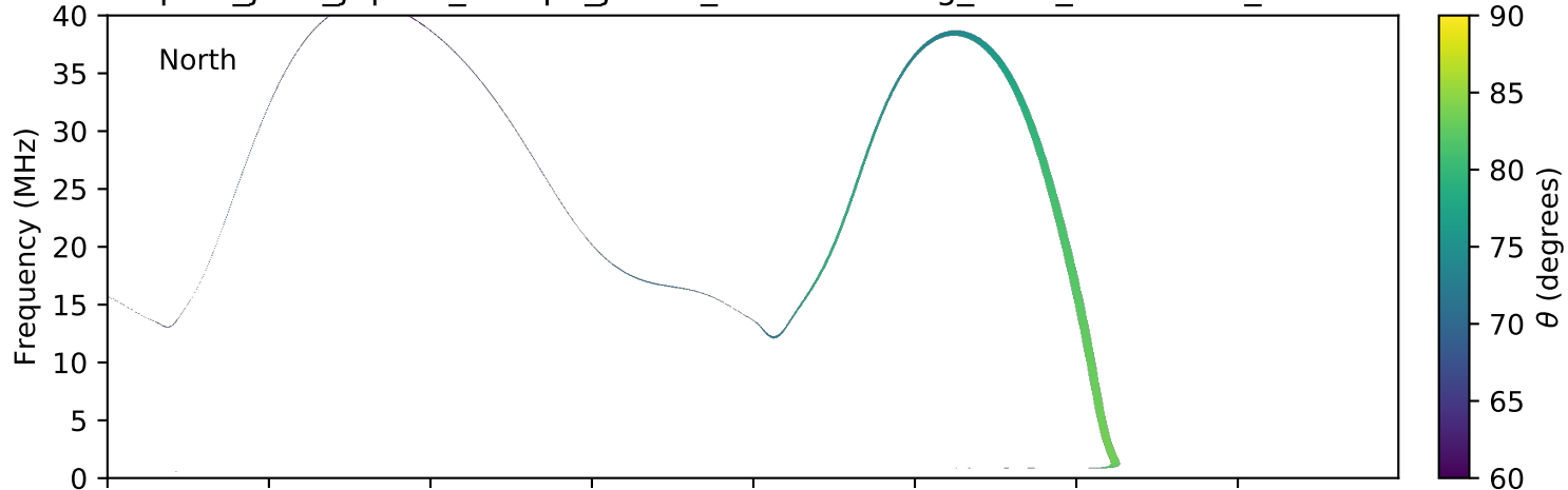
expres_juno_jupiter_europa_jrm09_lossc-wid1deg_3kev_20160814_v01.cdf
