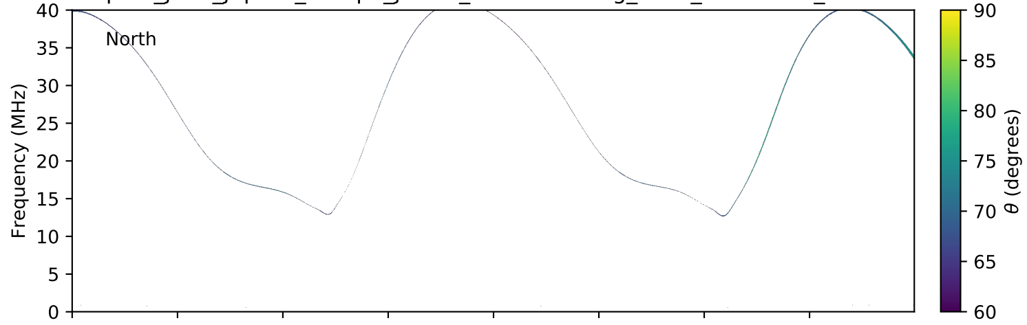
expres_juno_jupiter_europa_jrm09_lossc-wid1deg_3kev_20160810_v01.cdf
