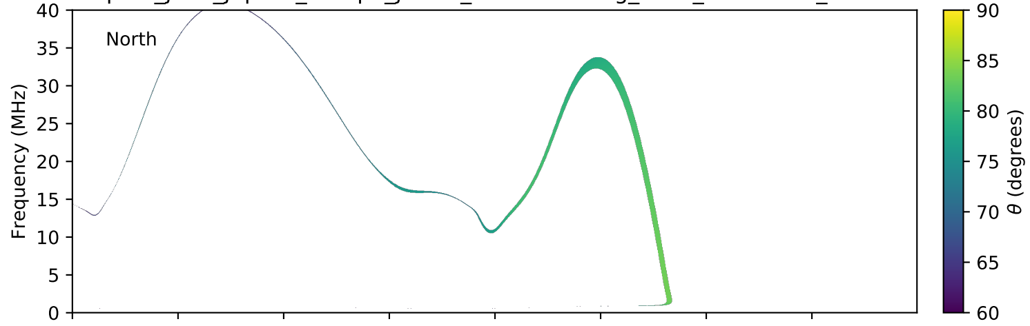
expres_juno_jupiter_europa_jrm09_lossc-wid1deg_3kev_20160807_v01.cdf
