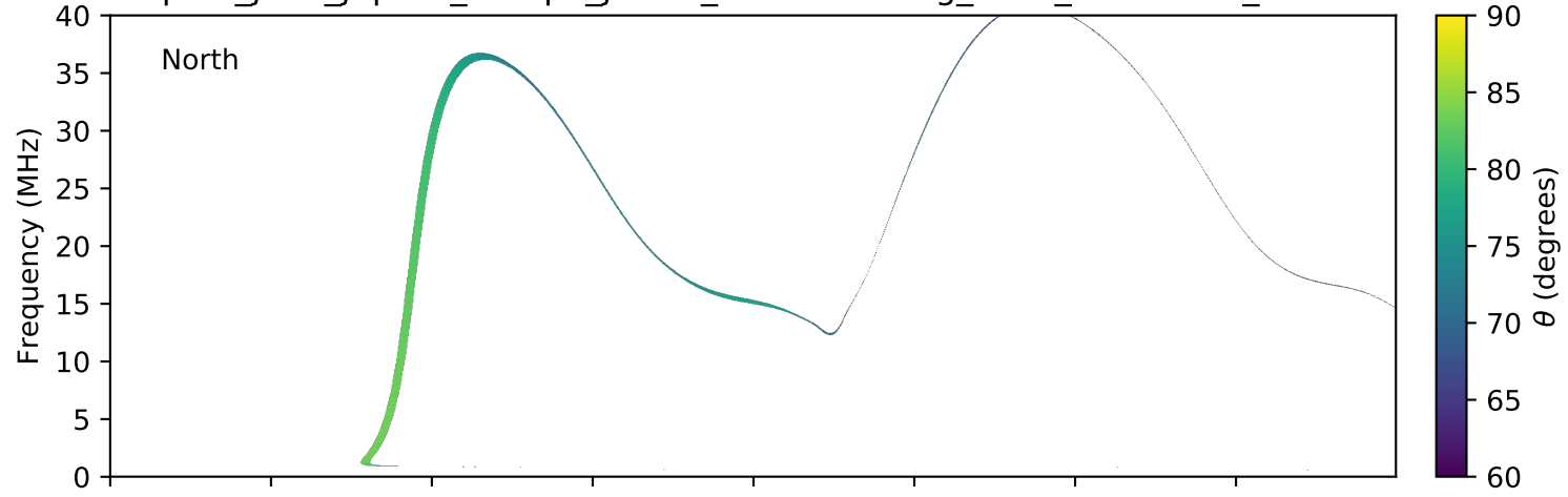
expres_juno_jupiter_europa_jrm09_lossc-wid1deg_3kev_20160806_v01.cdf
