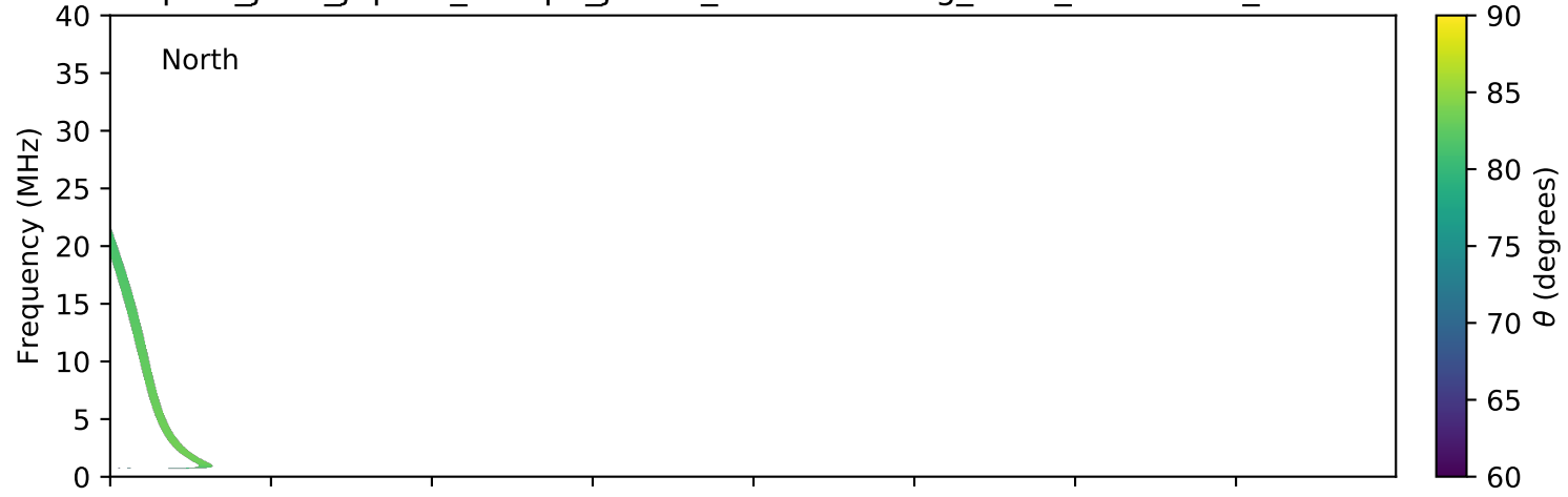
expres_juno_jupiter_europa_jrm09_lossc-wid1deg_3kev_20160804_v01.cdf
