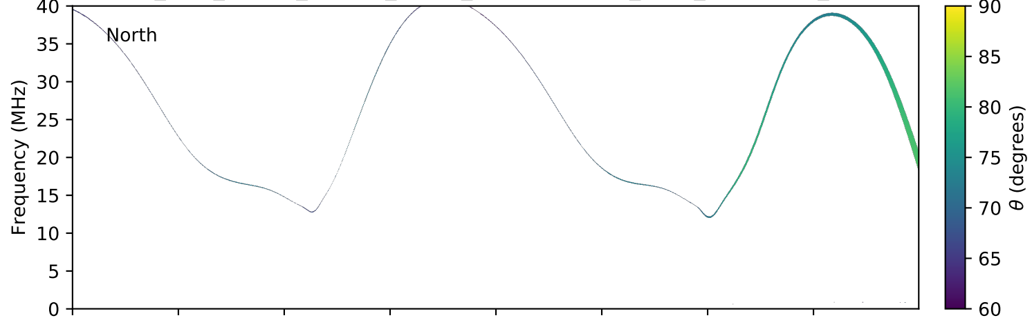
expres_juno_jupiter_europa_jrm09_lossc-wid1deg_3kev_20160803_v01.cdf
