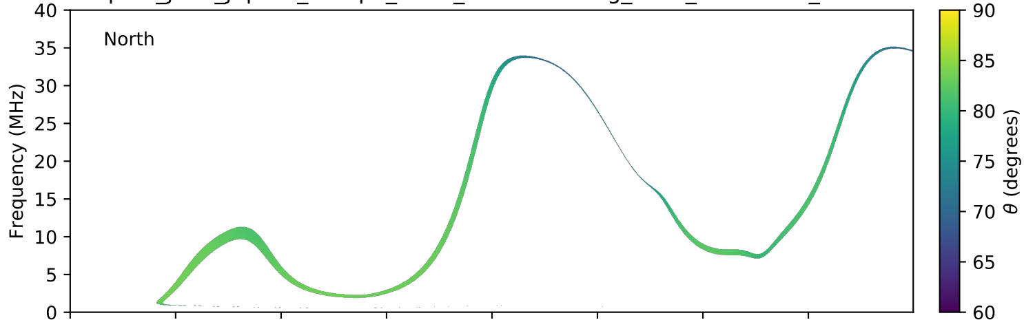
expres_juno_jupiter_europa_isaac_lossc-wid1deg_3kev_20160831_v01.cdf
