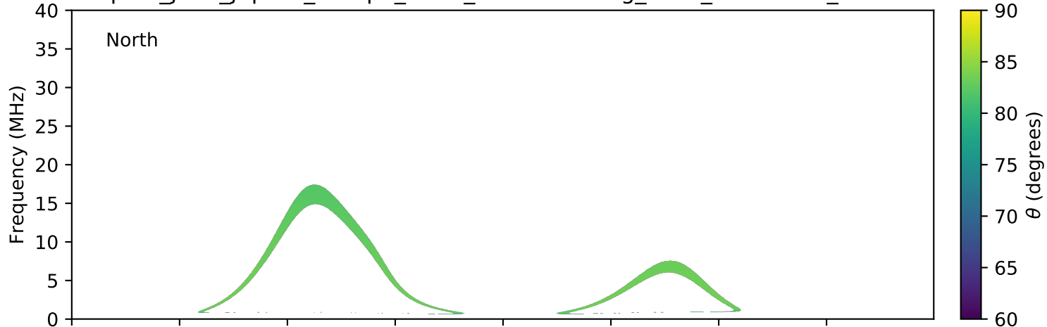
expres_juno_jupiter_europa_isaac_lossc-wid1deg_3kev_20160828_v01.cdf
