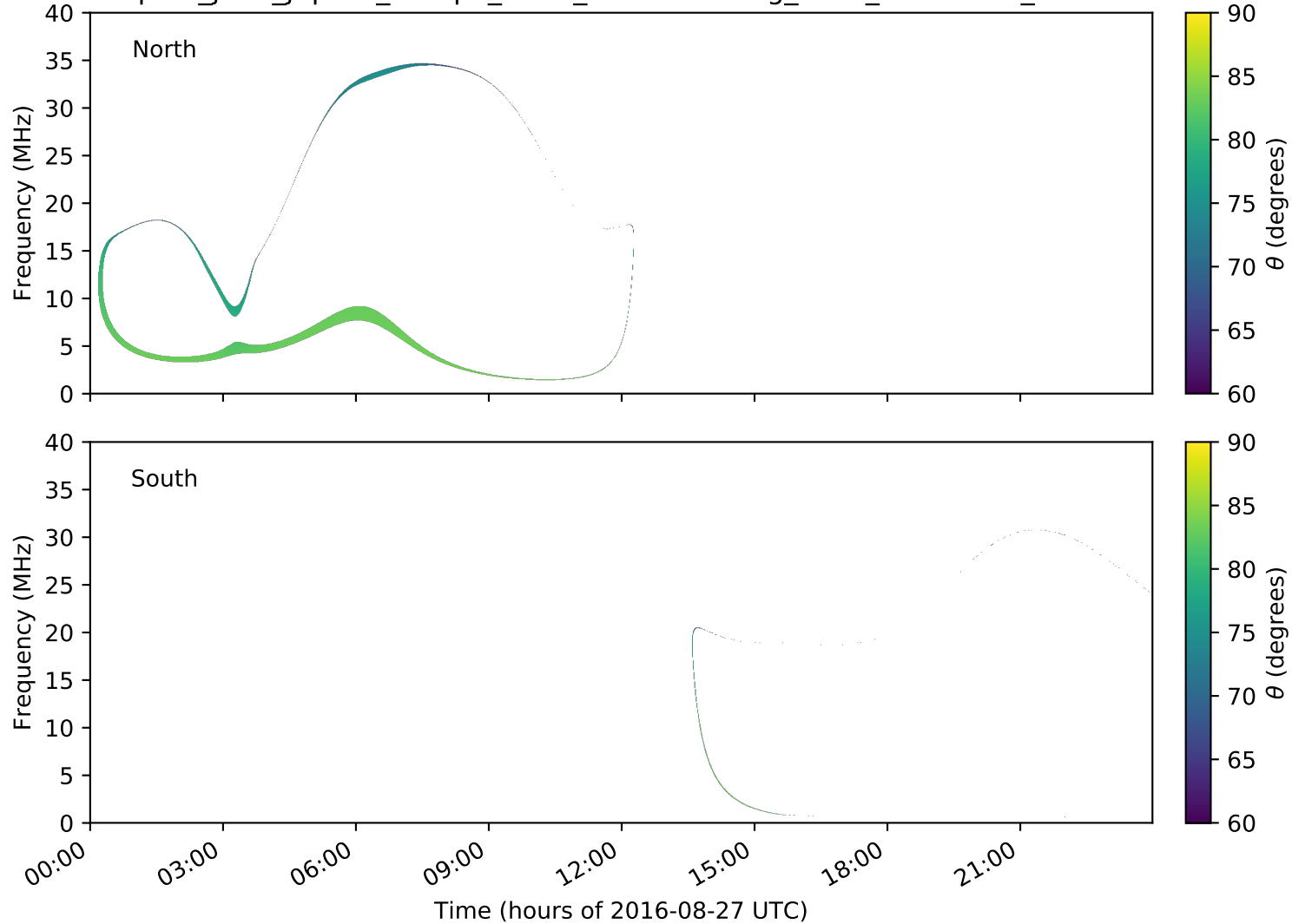
expres_juno_jupiter_europa_isaac_lossc-wid1deg_3kev_20160827_v01.cdf
