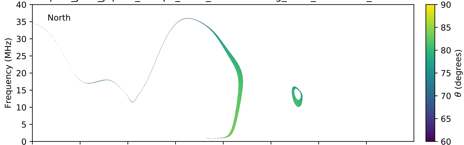
expres_juno_jupiter_europa_isaac_lossc-wid1deg_3kev_20160825_v01.cdf
