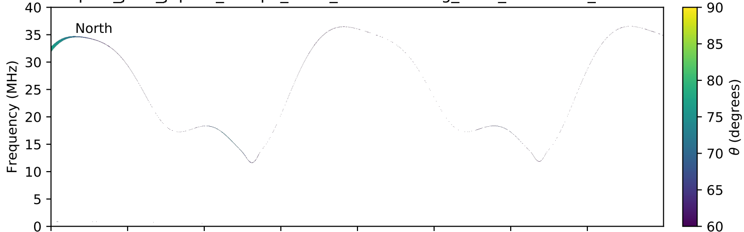
expres_juno_jupiter_europa_isaac_lossc-wid1deg_3kev_20160824_v01.cdf
