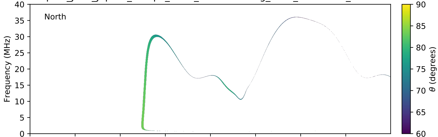
expres_juno_jupiter_europa_isaac_lossc-wid1deg_3kev_20160820_v01.cdf
