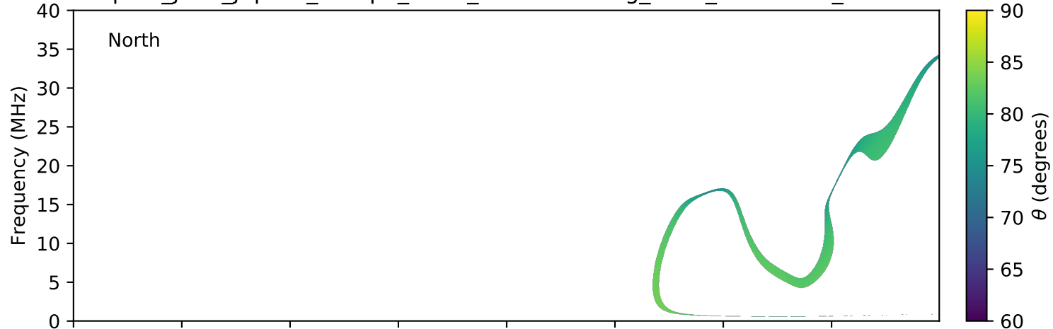
expres_juno_jupiter_europa_isaac_lossc-wid1deg_3kev_20160816_v01.cdf
