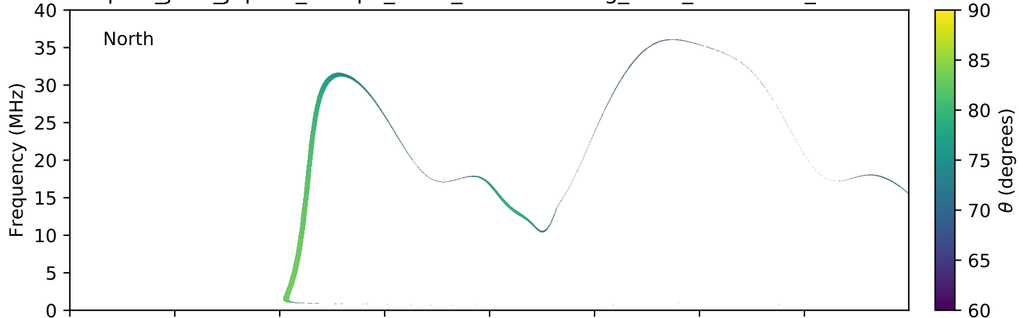
expres_juno_jupiter_europa_isaac_lossc-wid1deg_3kev_20160813_v01.cdf
