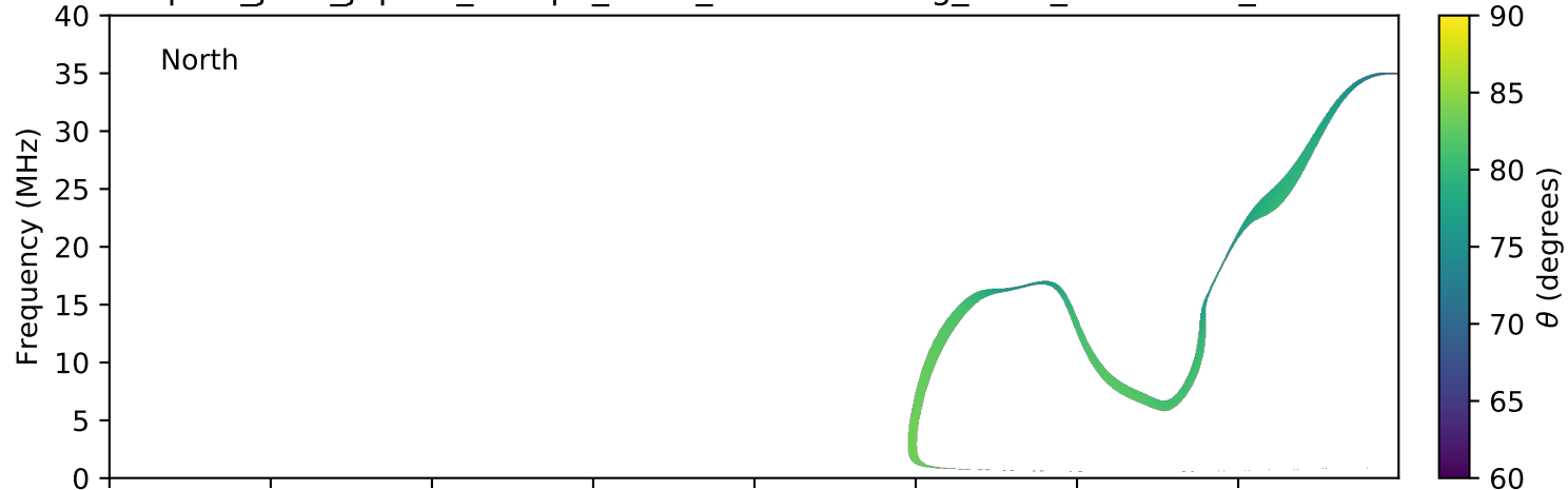
expres_juno_jupiter_europa_isaac_lossc-wid1deg_3kev_20160809_v01.cdf
