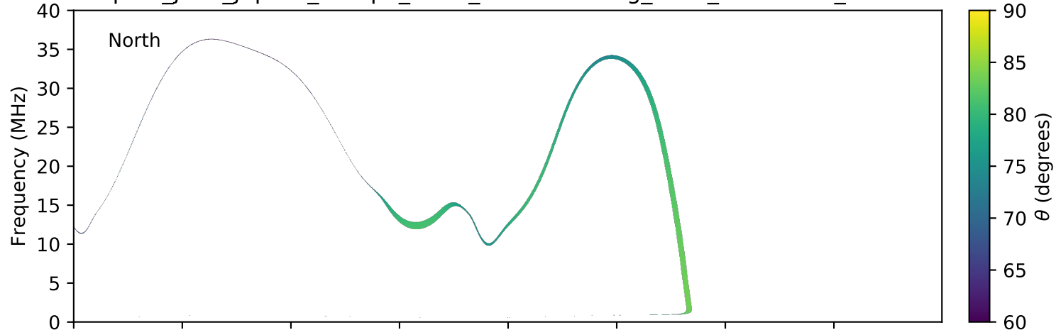
expres_juno_jupiter_europa_isaac_lossc-wid1deg_3kev_20160807_v01.cdf
