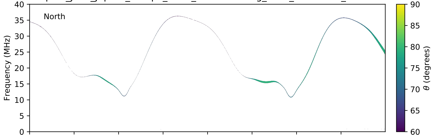
expres_juno_jupiter_europa_isaac_lossc-wid1deg_3kev_20160803_v01.cdf
