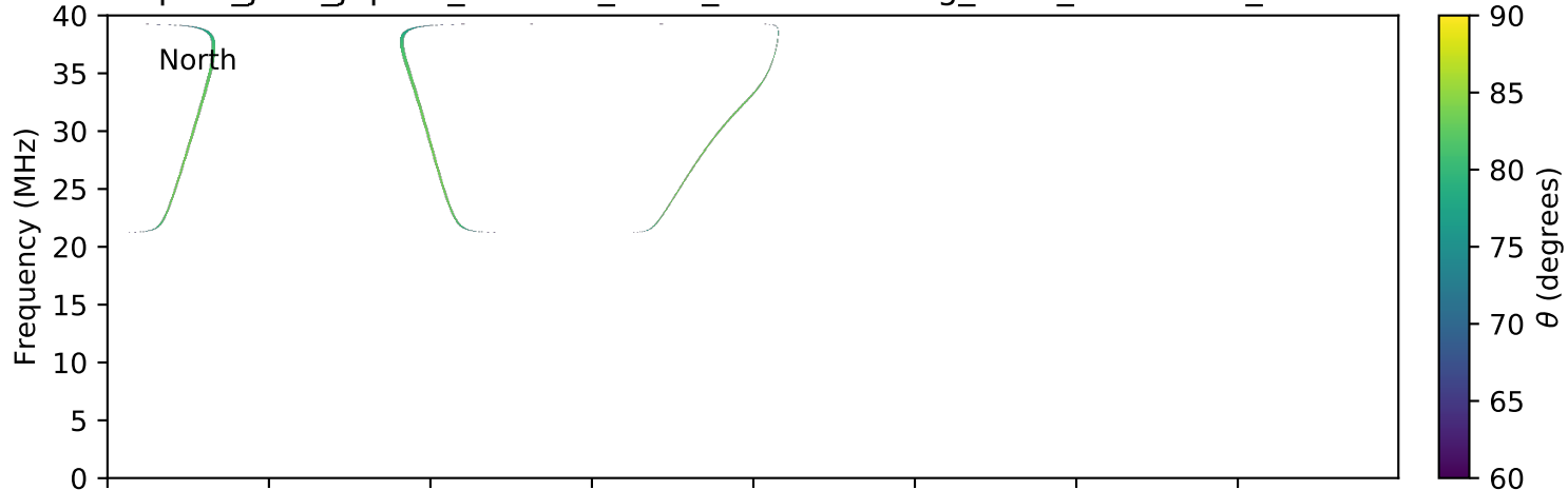
expres_juno_jupiter_118d-0r_isaac_lossc-wid1deg_3kev_20160827_v01.cdf
