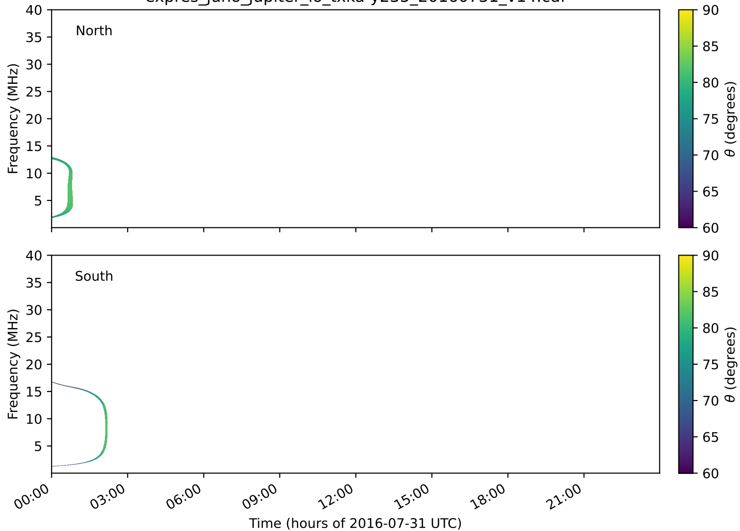
expres_juno_jupiter_io_txka-y235_20160731_v14.cdf
