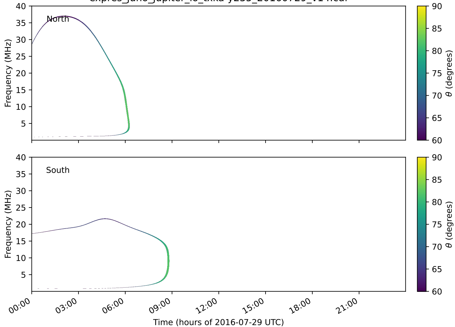
expres_juno_jupiter_io_txka-y235_20160729_v14.cdf
